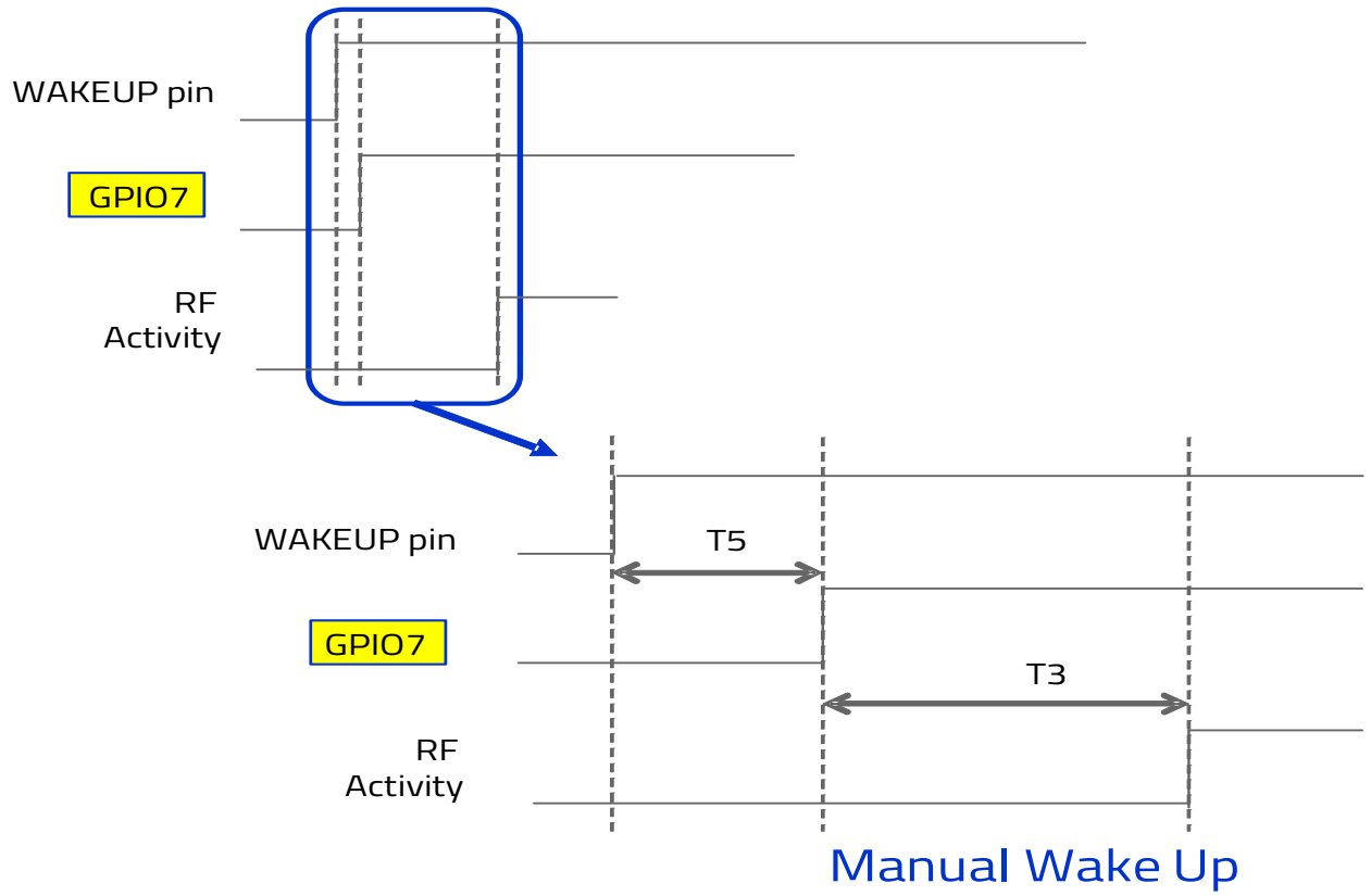
Figure 4-3: GPIO7 Waveform—Manual Wake Up
