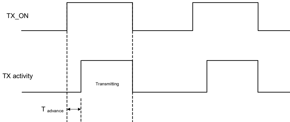
Figure 4-13: TX_ON State High during TX Activity
