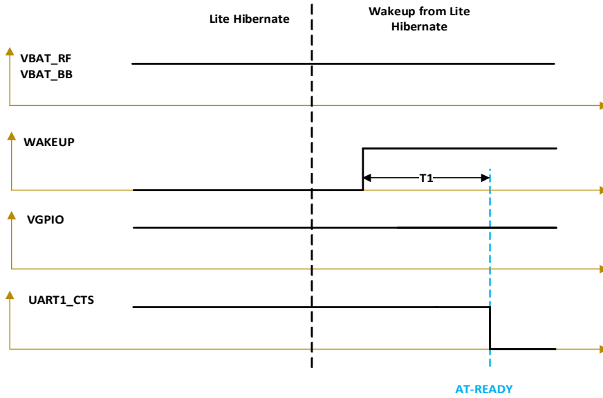
Figure 4-11: Wake up from Lite Hibernate Mode
