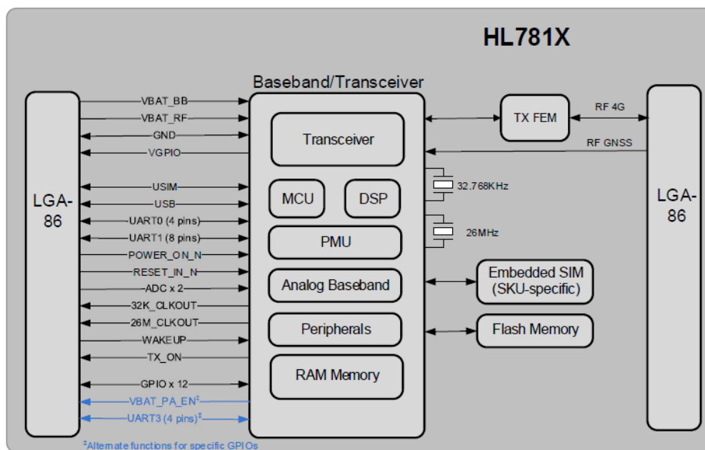
Figure 1-2: Architecture Overview
