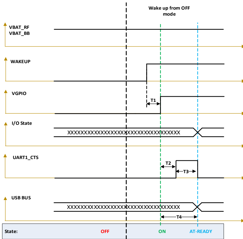
Figure 4-10: Wake up from OFF Mode
