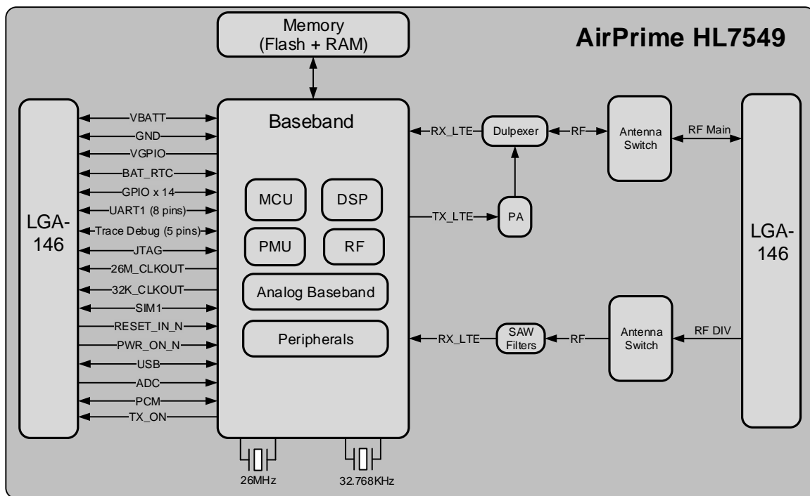
Figure 1. Architecture Overview
