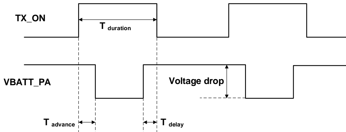
Figure 6. TX_ON State during Transmission
