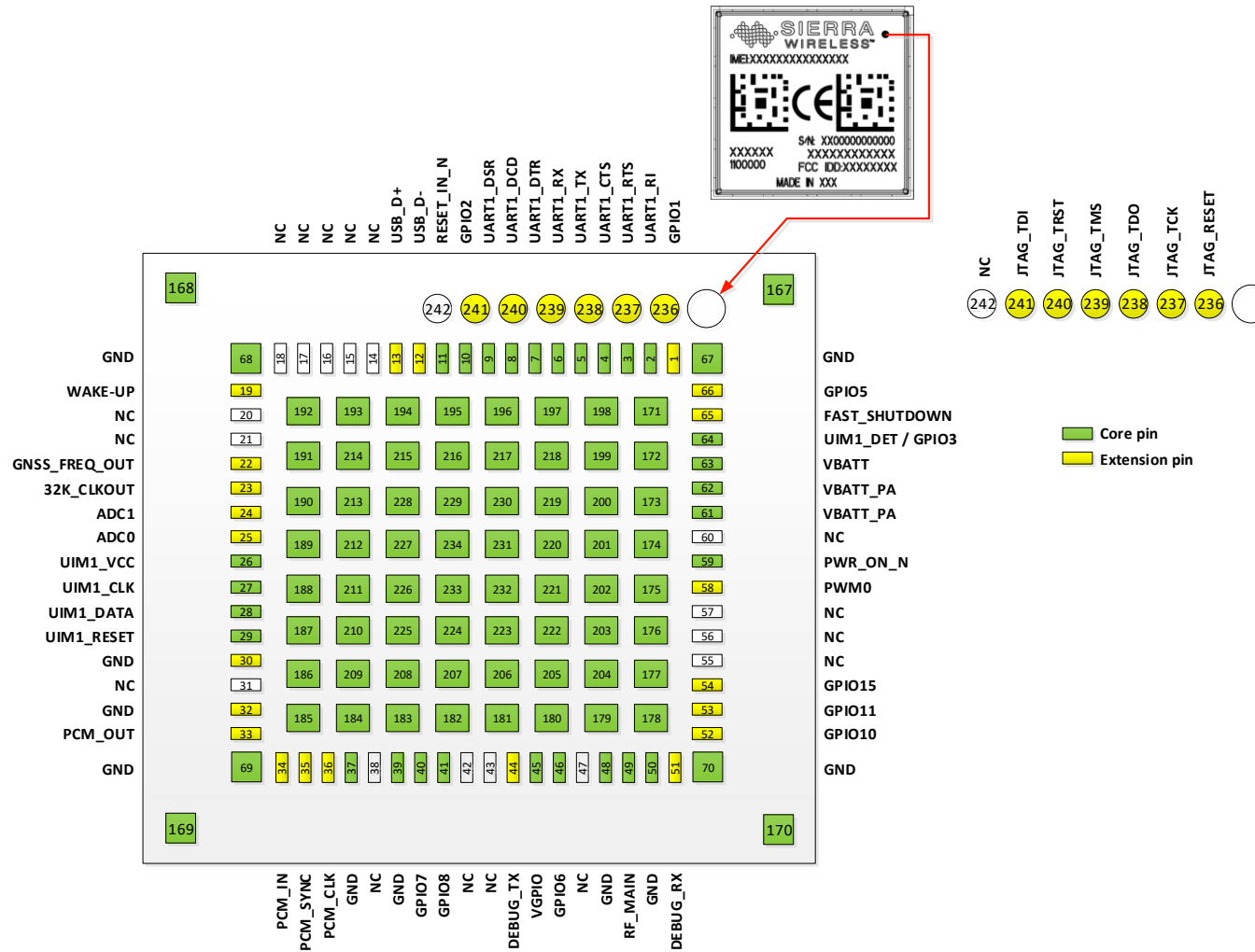
Figure 5. Pad Configuration
