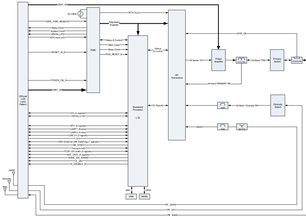
Figure 2-1: RC7611, RC7611-1, RC7611D, RC7611D-1, RC7612*, RC7612-1*, RC7630, RC7630-1, RC7630J* Architecture Overview
