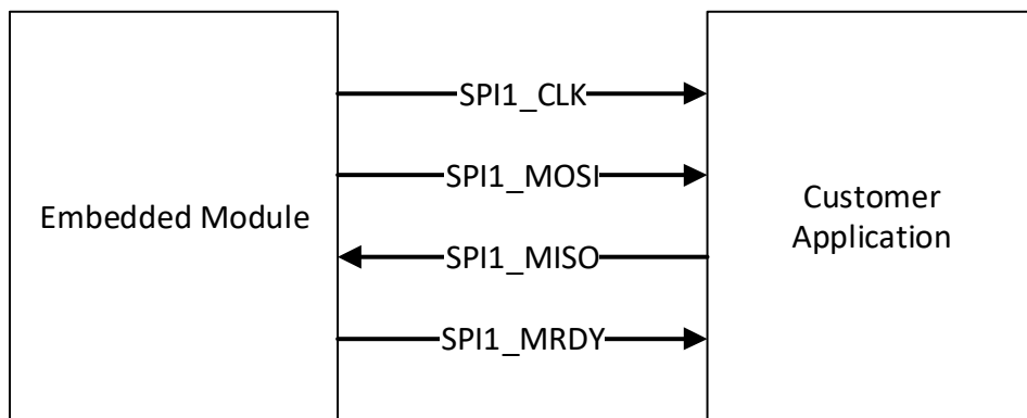
Figure 4-28: Example of 4-wire SPI Bus Application
