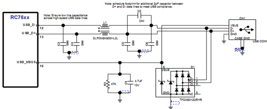
Figure 5-10: USB Interface
