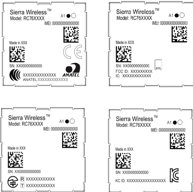
Figure 6-1: Unit Product Marking—Laser-etched, Typical Representation
