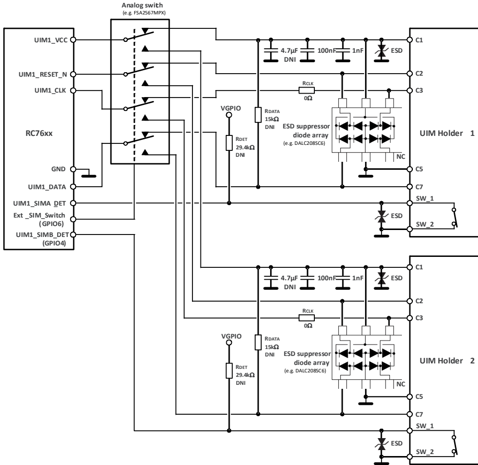
Figure 5-9: External SIM schematic for RC7611, RC7611D, RC7620, RC7630, and RC7630J* * Limited availability
