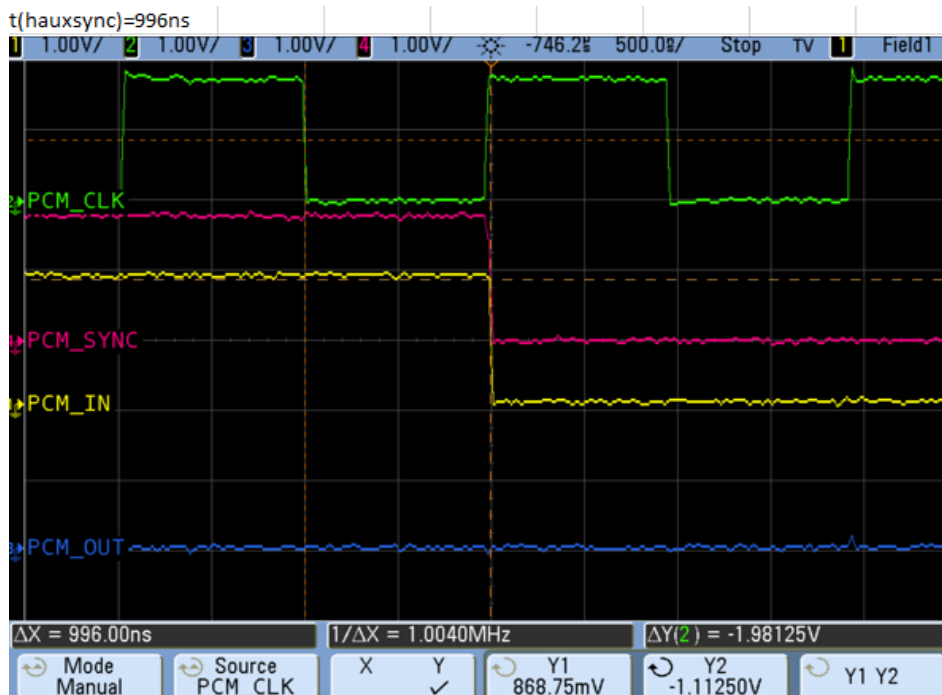
Figure 4-15: t(hauxsync)
