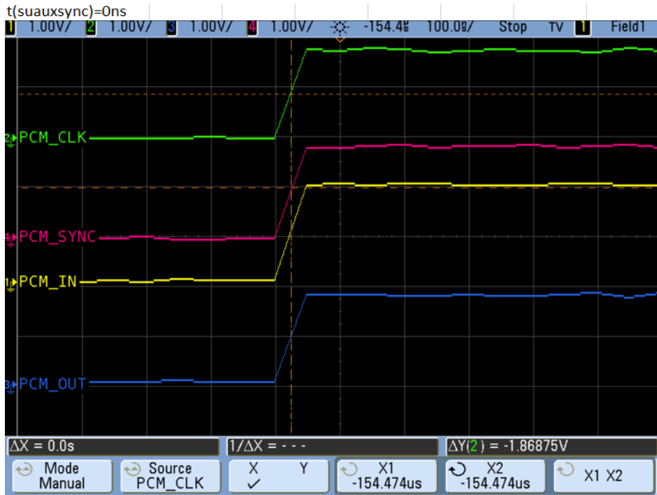
Figure 4-18: t(susync)
