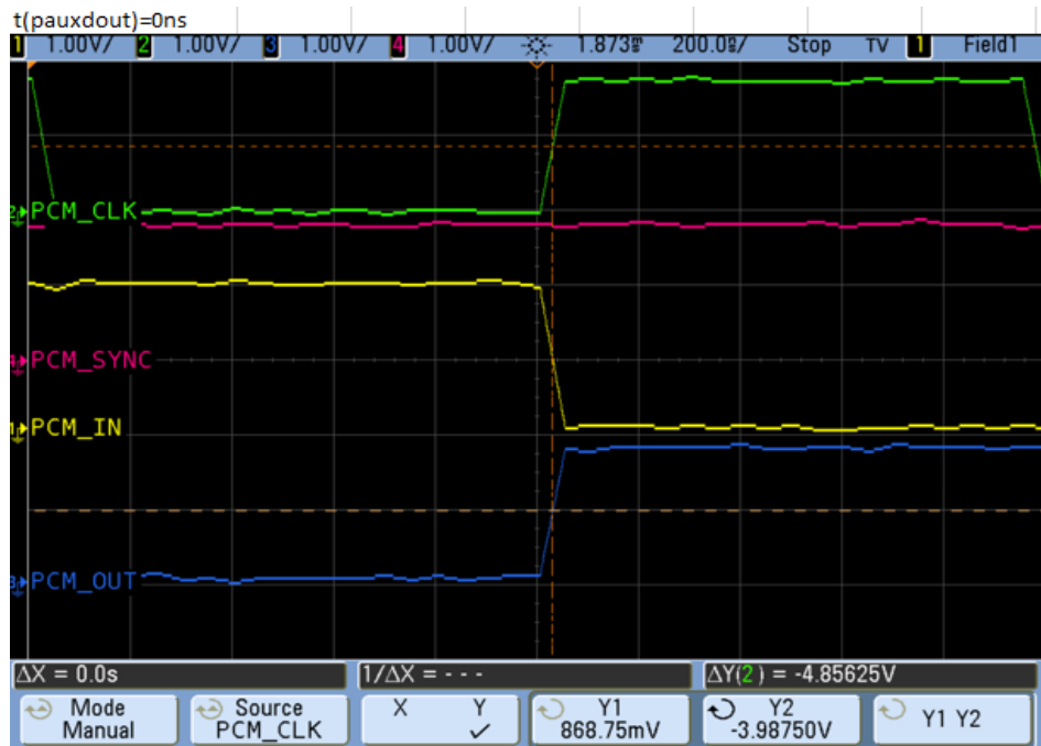
Figure 4-23: t(\text{pauxdout})
