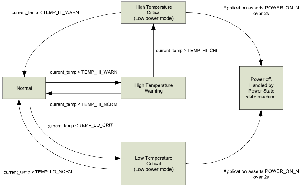
Figure 4-29: Temperature Monitoring State Machine
