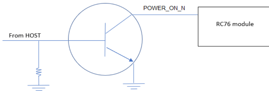
Figure 4-1: POWER_ON_N
