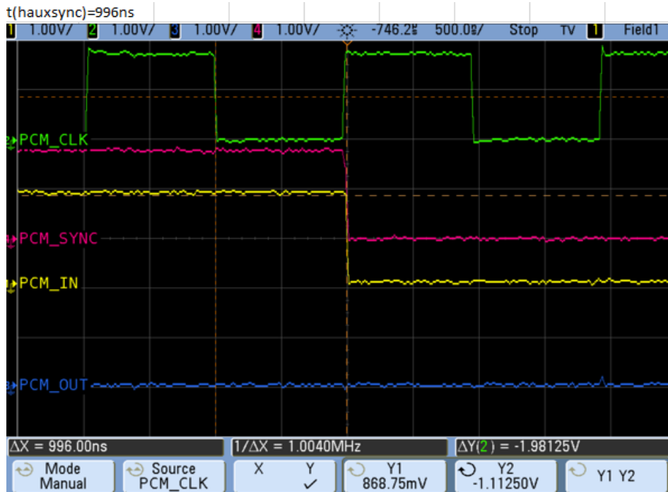
Figure 4-22: t(\text{hauxsync})
