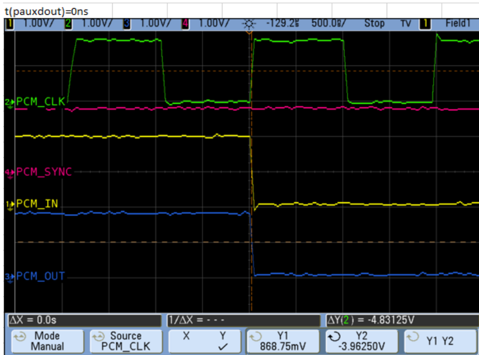
Figure 4-24: t(pauxdout)R
