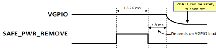
Figure 4-33: SAFE_PWR_REMOVE
