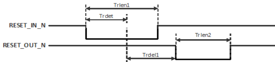
Figure 4-7: Reset timing when RESET_IN_N < Trdel1
