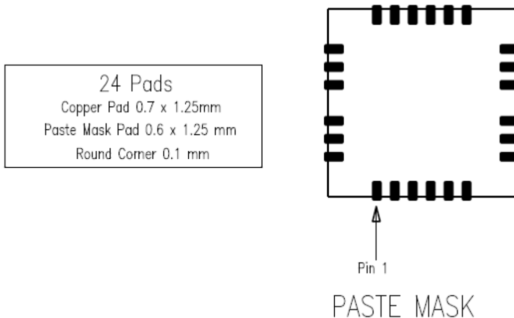
Figure 7. Recommended Paste Mask Layout
