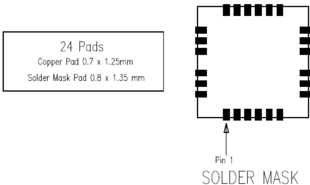
Figure 6. Recommended Solder Mask
