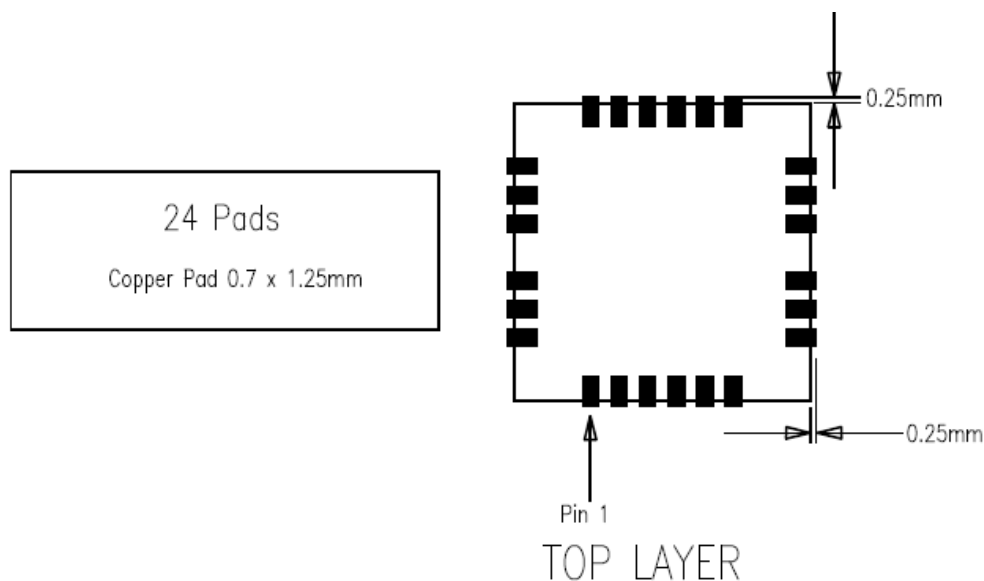
Figure 5. Recommended Footprint – Copper Layout
