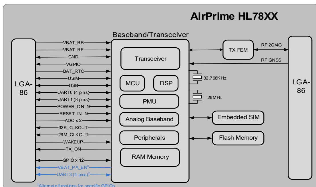
Figure 1-2: Architecture Overview
