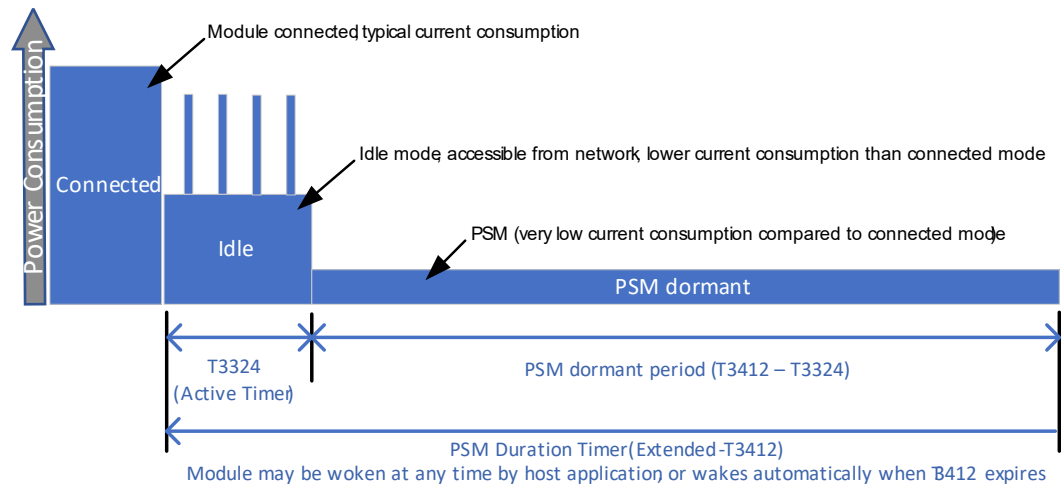
Figure 3-1: PSM—Timers
