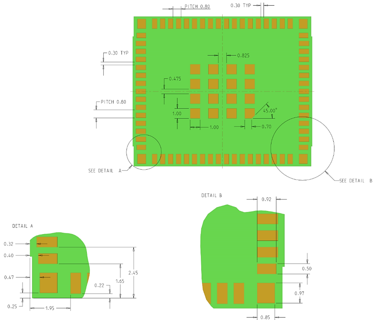
Figure 5-2: Dimensions Drawing
