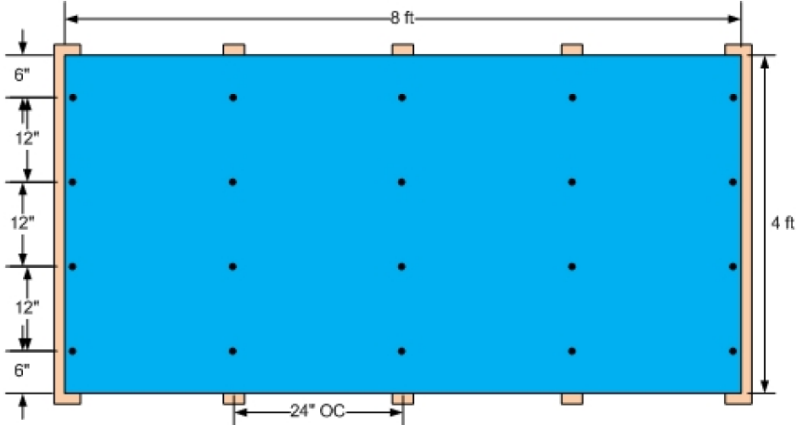
Figure 1, Fastening Configurations, Exposed Fastening (continued)
