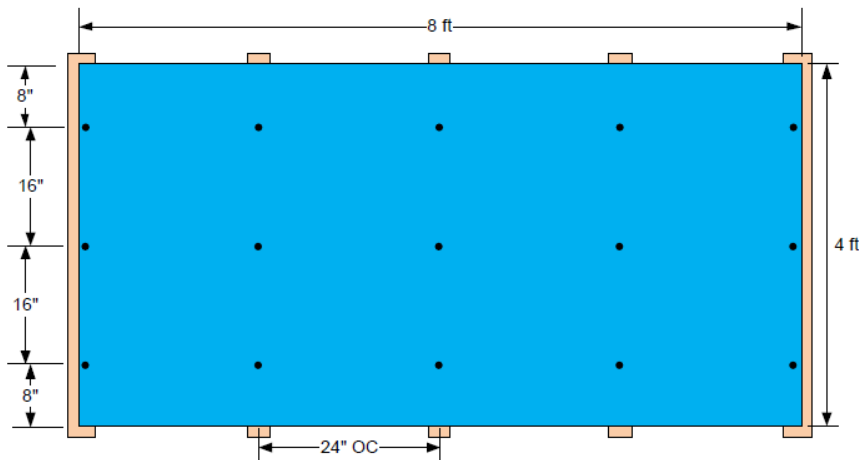
Configuration 11 (Countersunk): 24" OC Steel Stud Frame
