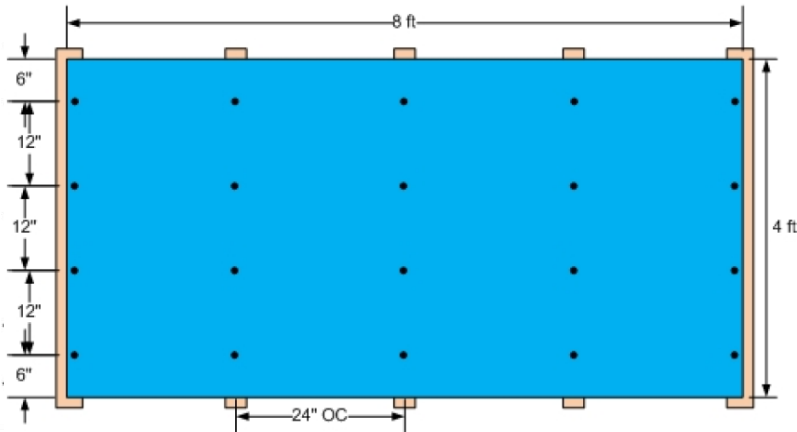
Configuration 6 (Exposed): 24" OC Steel Stud Frame
