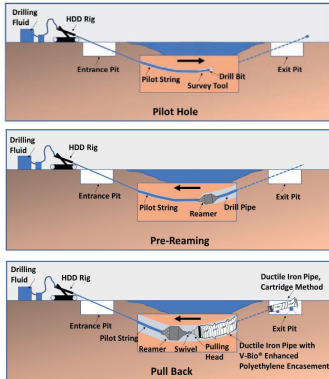
Figure 3: HDD Stages
