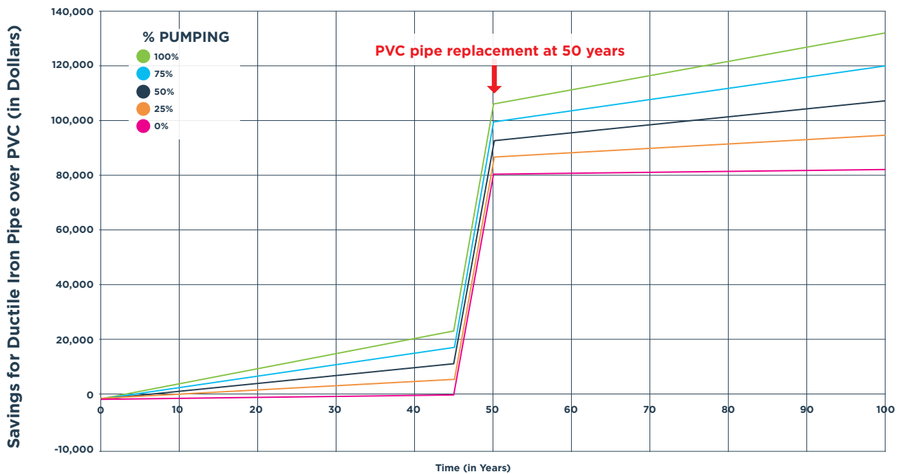
Ductile Iron Pipe over PVC (24" Diameter)
