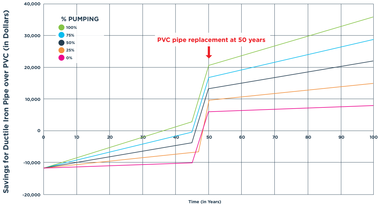
Ductile Iron Pipe over PVC (24" Diameter)
