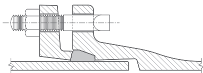
MECHANICAL JOINT
