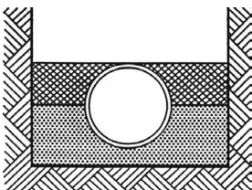
Type 5 Pipe bedded to its centerline in compacted granular material, ** 4-inch minimum under pipe. Compacted granular or select ‡ material to top of pipe. (Approximately 90% Standard Proctor, AASHTO T-99.) §
