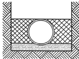
Type 4 Pipe bedded in sand, gravel, or crushed stone to depth of 1/8 pipe diameter, 4-inch minimum. Backfill compacted to top of pipe. (Approximately 80% Standard Proctor, AASHTO T-99.) § (See Table 1 for notes.)
