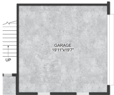
OPT 2-CAR SIDE ENTRY GARAGE
