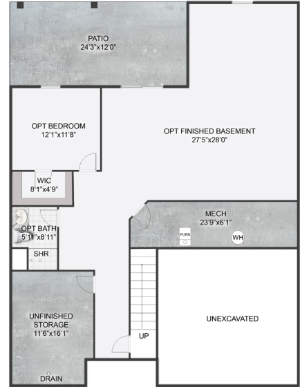
DECK W/ OPT LUXURY REAR WALKOUT FOUNDATION PLAN
