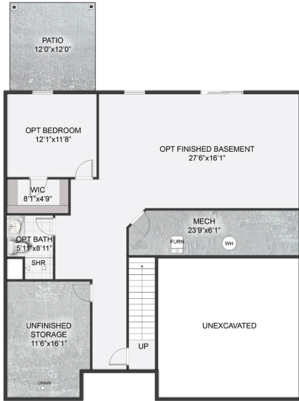
OPT LUXURY REAR WALKOUT FOUNDATION PLAN
