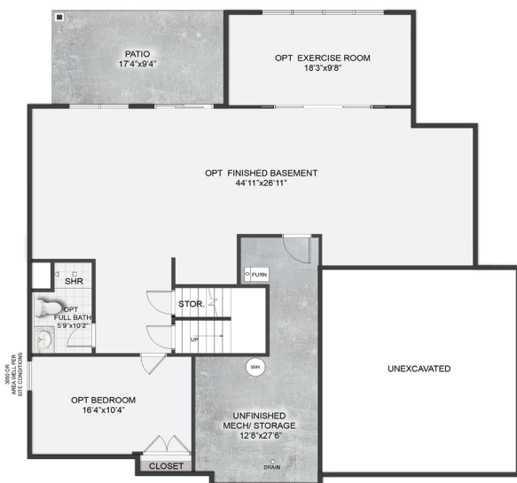
OPT LUXURY REAR WALKOUT FOUNDATION PLAN W/ OPT FINISHED BASEMENT
