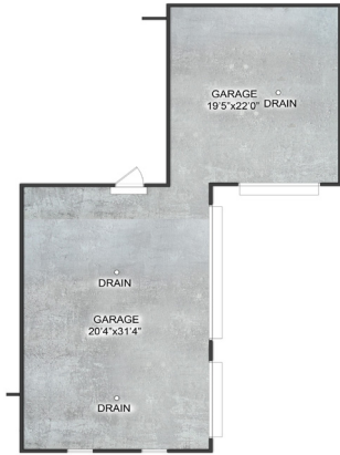
OPT 4 CAR SPLIT ENTRY GARAGE
