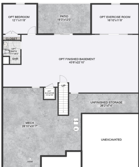
OPT SIGNATURE REAR WALKOUT FOUNDATION PLAN W/ OPT FINISHED BASEMENT
