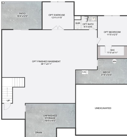
OPT SIGNATURE REAR WALKOUT FOUNDATION PLAN W/ OPT FINISHED BASEMENT
