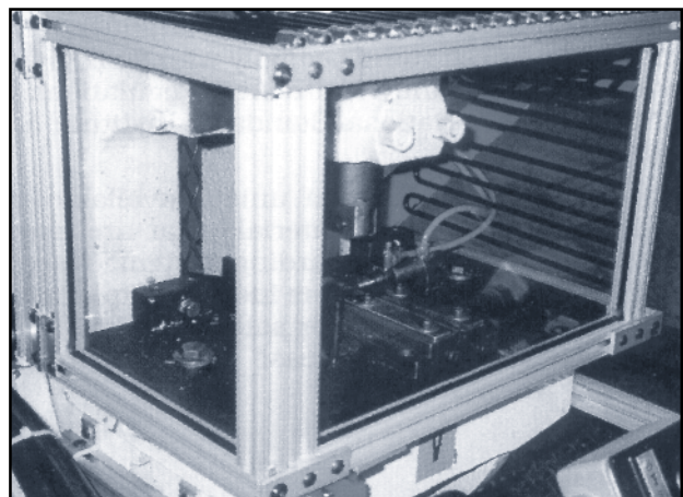
Barrier guarding on an OBI mechanical power press.
