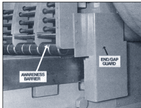
If the C-frame throat is open on either side of a power squaring shear, the gap must be guarded. Cincinnati Inc.
