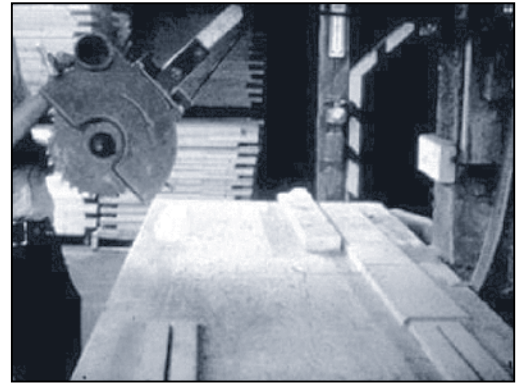
Overhead swing saw missing a lower blade guard and extending beyond table edge.
