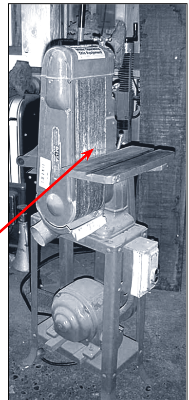
Nip point
