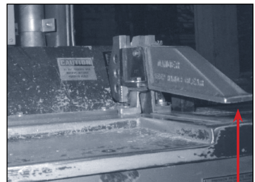
Missing “nose guard” on a jump saw.
