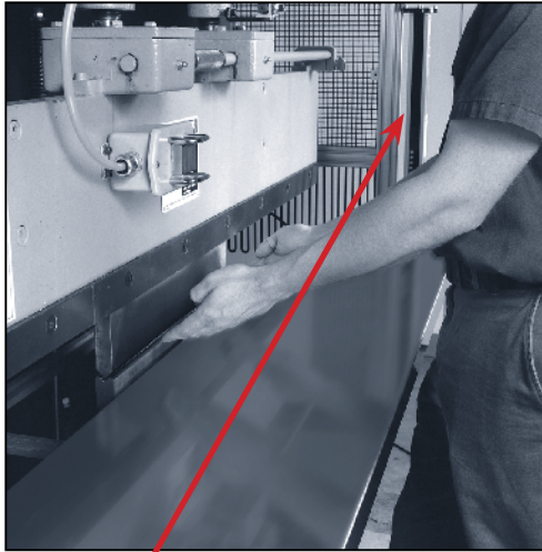
Rockford Systems Inc. Presence-sensing device (light curtain) used.
