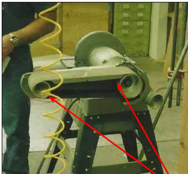
Belt sander missing guards over in-running nip points and belt edge.
