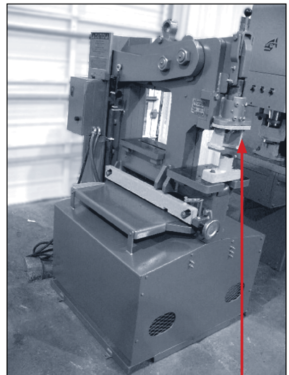
“Strippers” are designed to hold the material down and may also provide some protection from the punch hazard.
