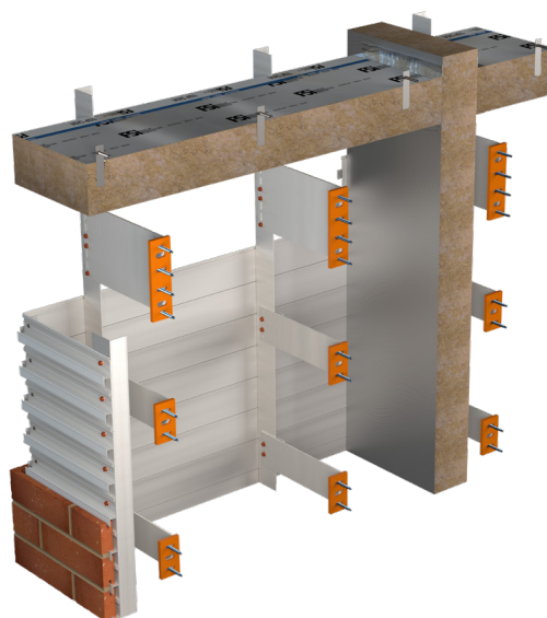
Briklok S (standard) for bricks 62 to 65mm in height
