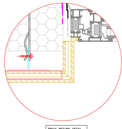
BRICK RETURN DETAIL
