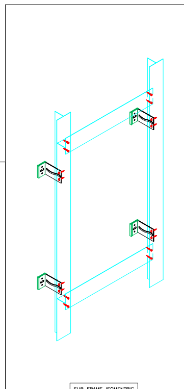
SUB FRAME ISOMETRIC
