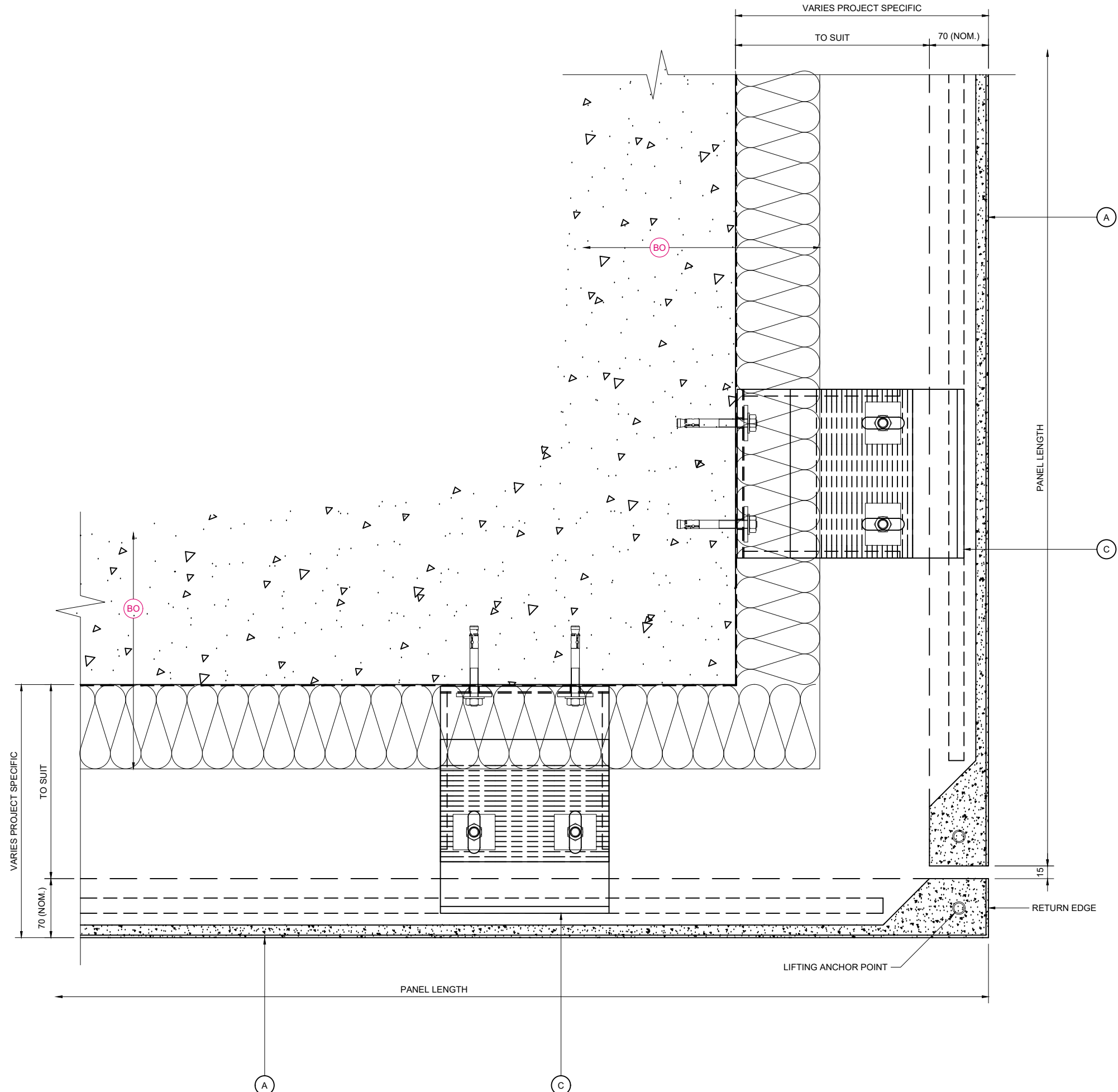
EXTERNAL CORNER DETAIL
