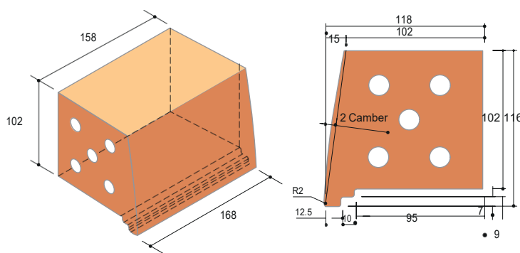
Tile Brick Profile (Perforation patterns may vary)
