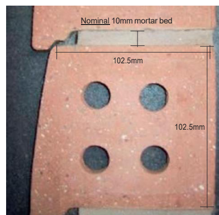
Tilebrick section showing bed joint mortar placement set approx 15mm back from top of Tilebrick unit. (Perforation platforms are likely to differ from picture).
