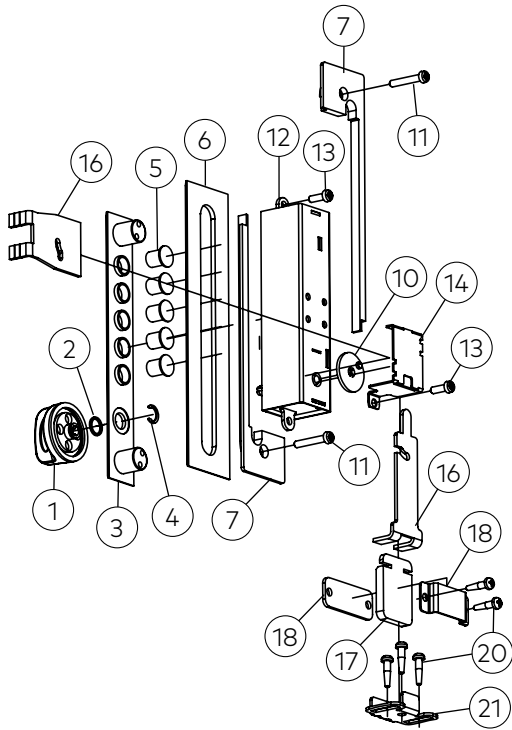
962 Wood/Deadbolt
