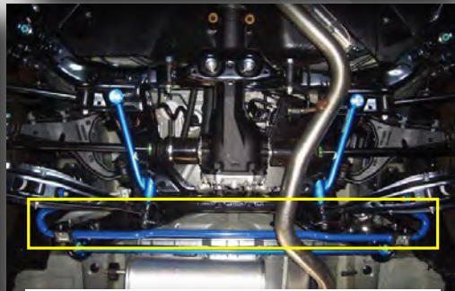
Rear Sway Bar (20mm) (GPE) Part No: 692 311 B20 MSRP: $347.00
