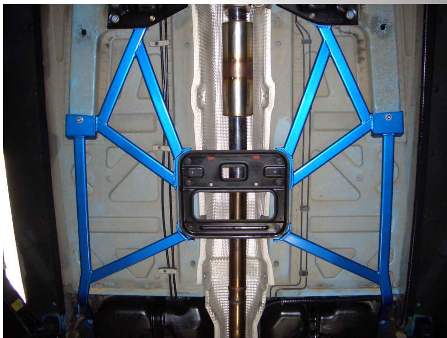
Undershot of mounting points front & rear power brace
