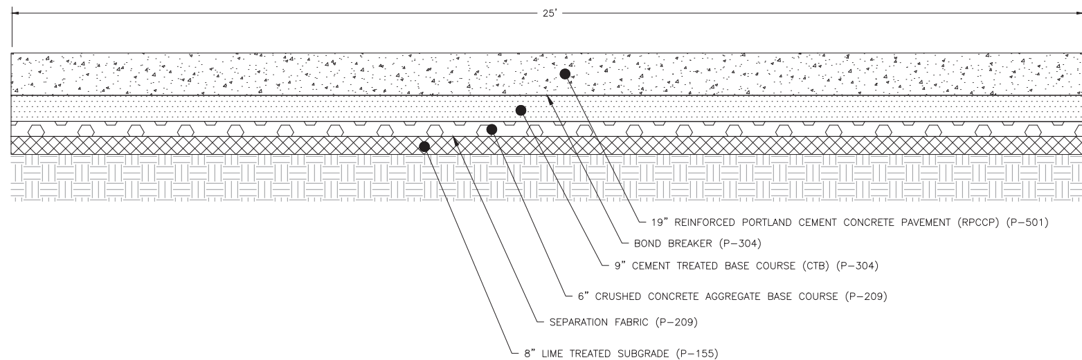
3 CP02.01 PROPOSED PAVEMENT SECTION - SOUTH SCALE: NTS
