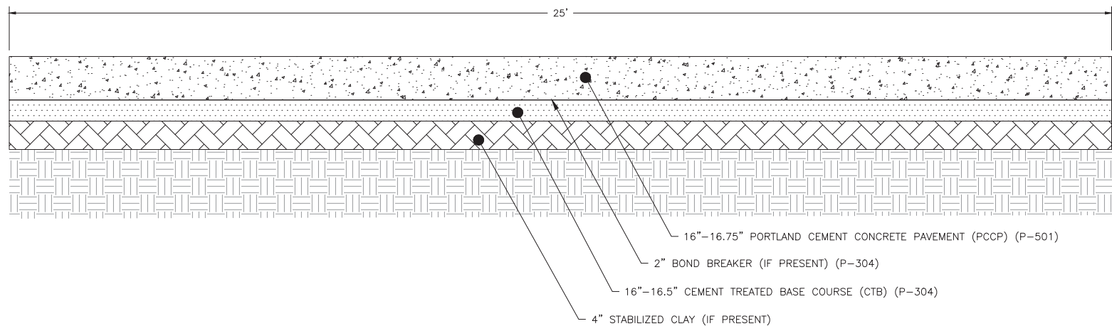
1 CP02.01 EXISTING PAVEMENT SECTION SCALE:NTS
