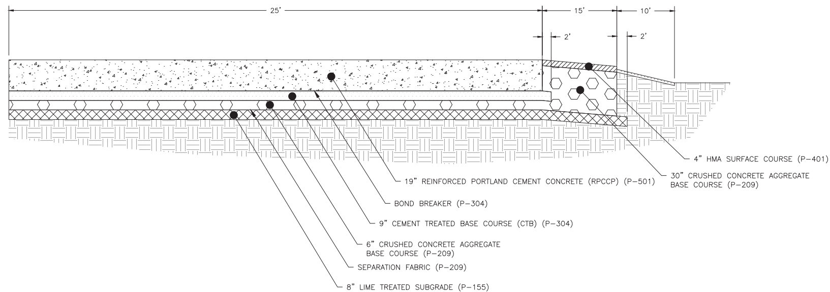
PROPOSED PAVEMENT SECTION - NORTH
