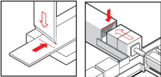
Figure 7 – Sliding hazards diagram
