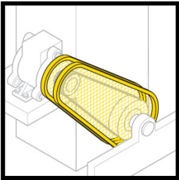
Figure 1 – Illustration of a belt and pulley safeguarded through implementation of a fixed guard
