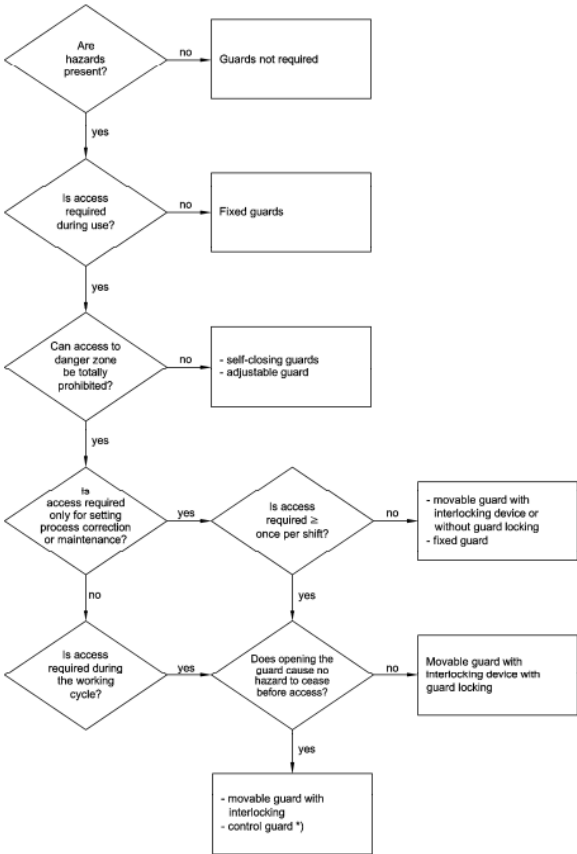
Figure 1: Selection Process of Guards
