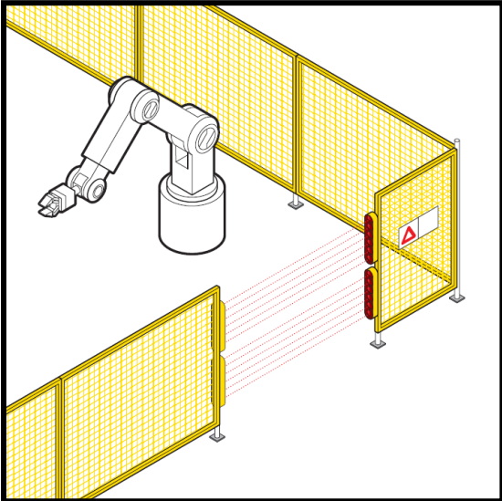
Figure 2 – Presence Sensing Equipment
