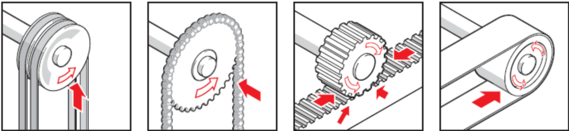
Figure 2 – Trapping hazards diagram
