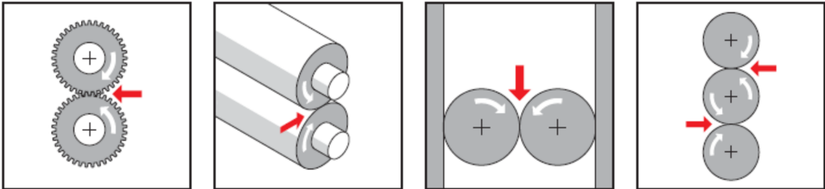
Figure 1 – Drawing hazards diagrams
