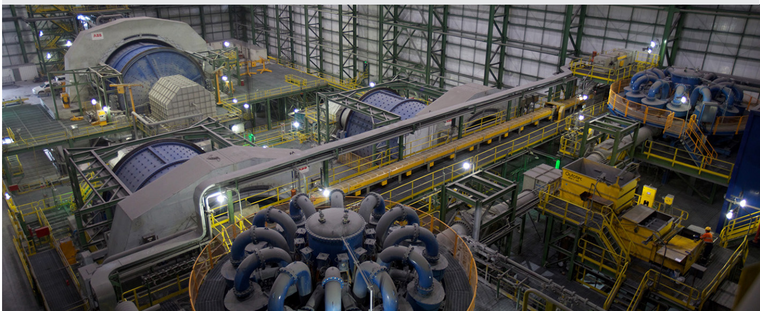
Image 2 – Aktogay Grinding Circuit
