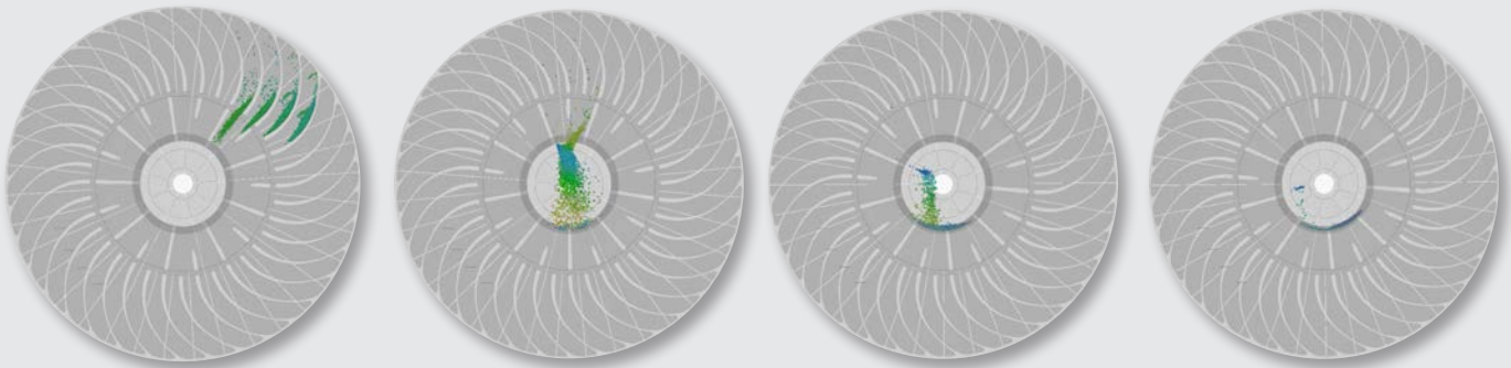
Figure 7 – DEM Results for the Super Vortex Discharge Design
