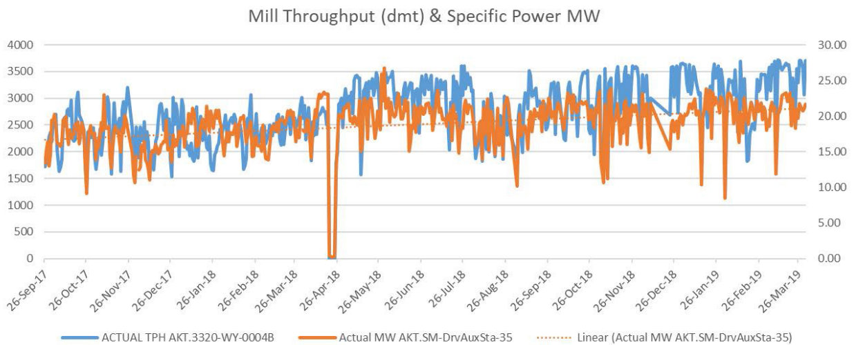
Figure 18 – SAG Mill Throughput and Specific Power
