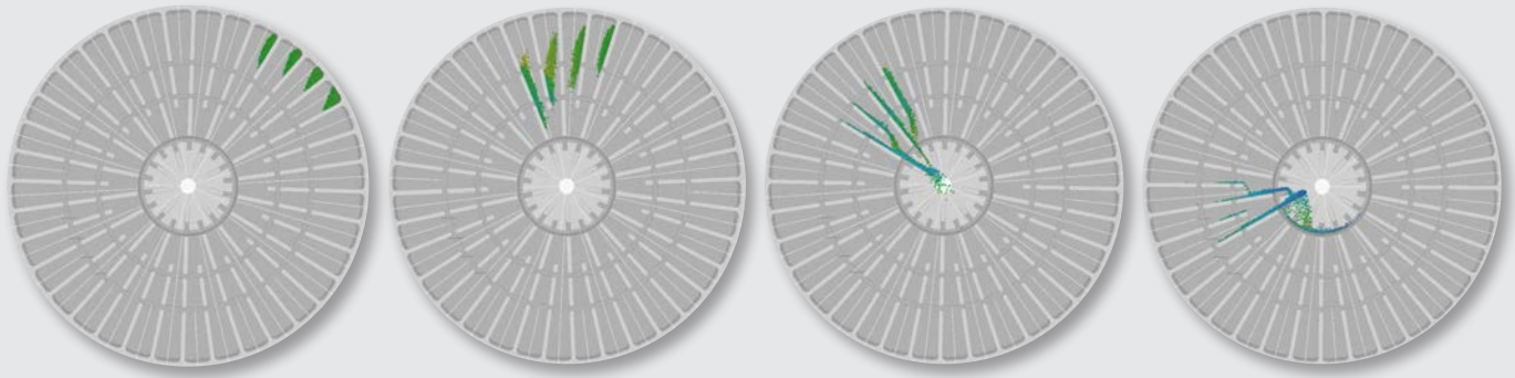
Figure 6 – DEM Results for the Straight Radial Discharge Design
