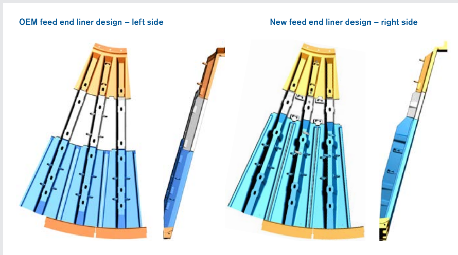
Figure 4 – Stage 1 Feed End Re-design Comparison
