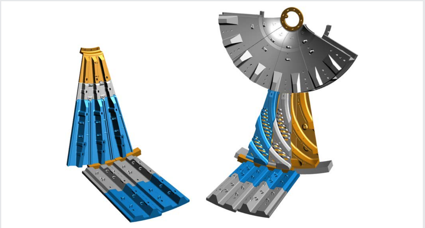
Figure 3 – Stage 1 Liner General Assembly
