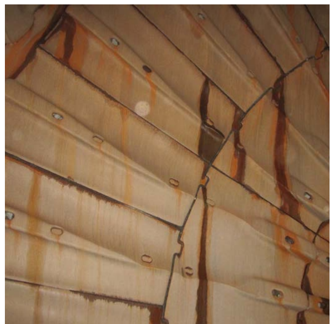
Image 3 – Feed End Liners showing High Wear Zone
