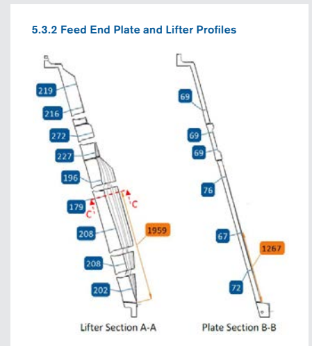
Figure 5 – New Feed End Outer Liner Wear Profile
