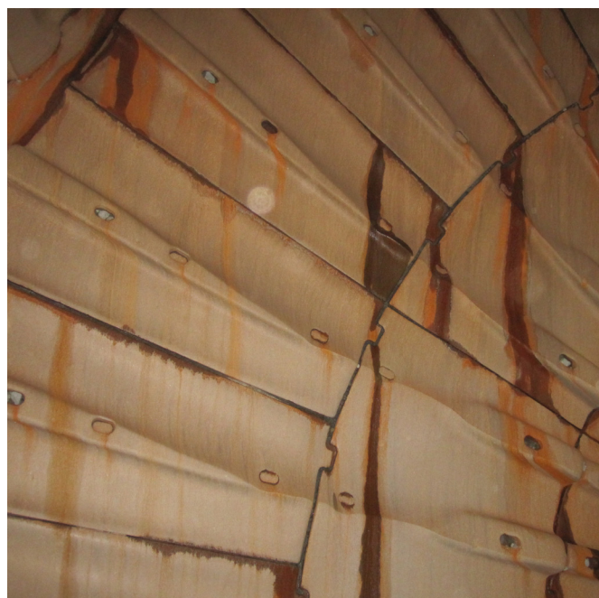
Image 3 – Feed End Liners showing High Wear Zone
