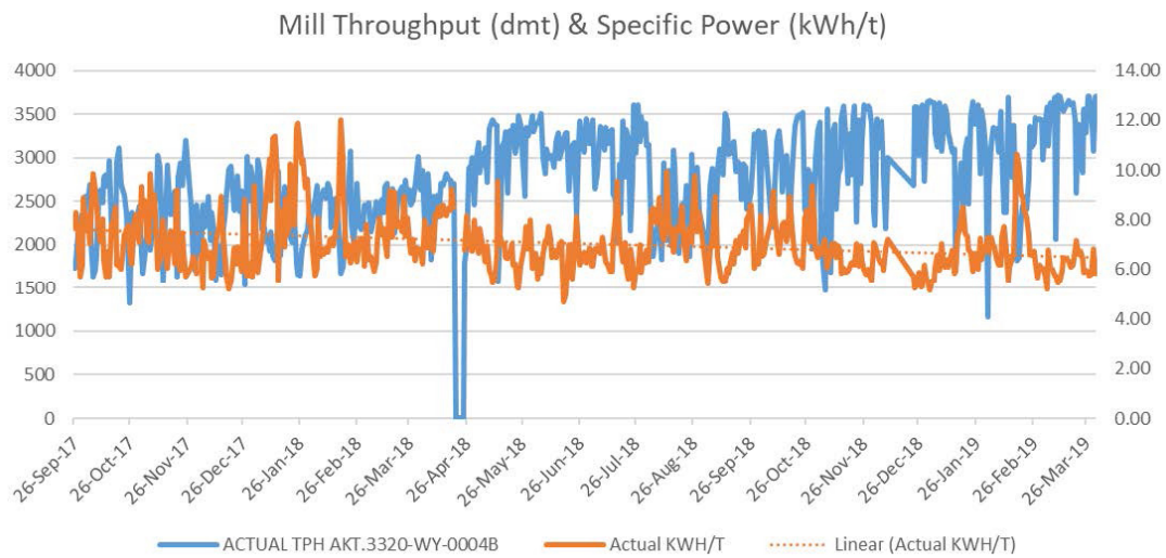
Figure 17 – SAG Mill Throughput and Specific Power kWh/t
