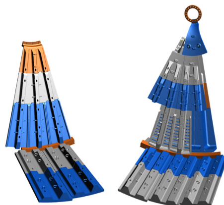
Figure 4 – OEM Liner Set General Assembly
