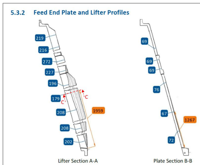
Figure 11 – New Feed End Outer Liner Wear Profile
