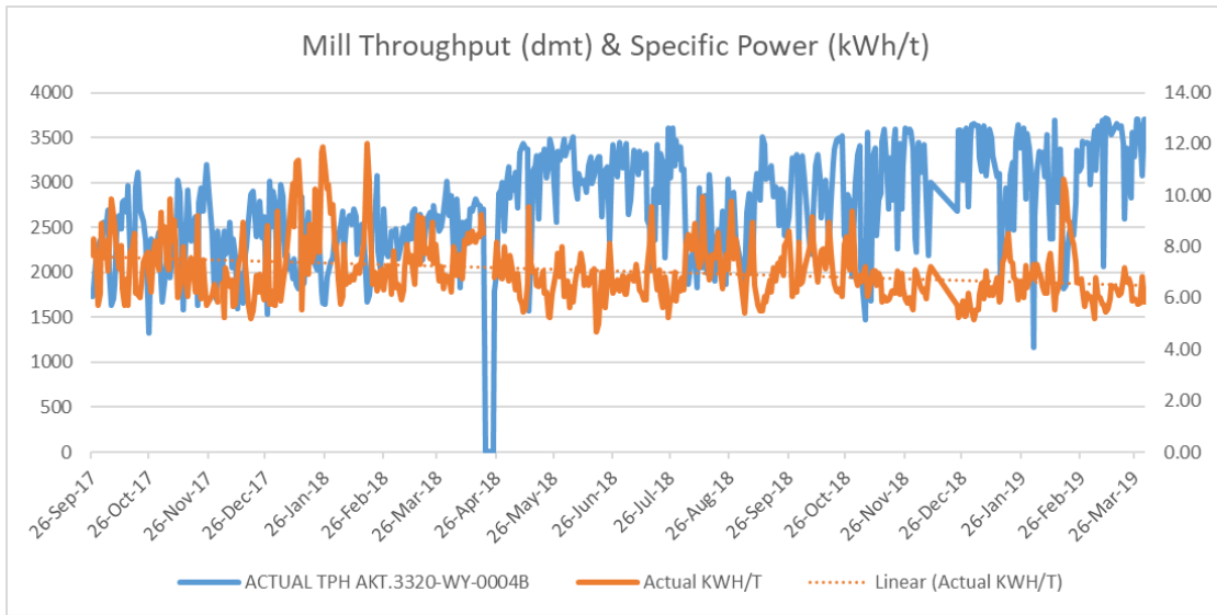
Figure 17 – SAG Mill Throughput and Specific Power kWh/t
