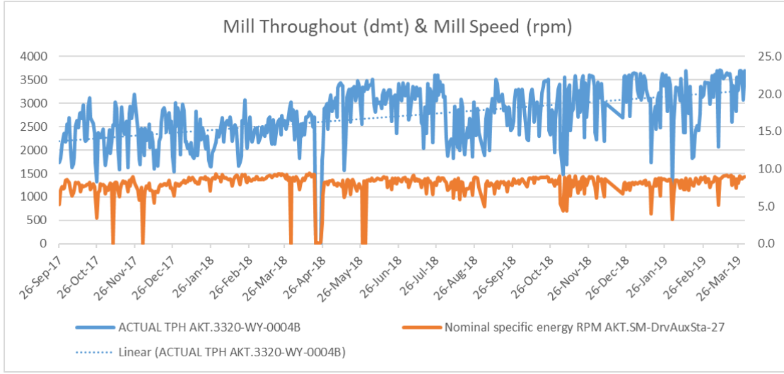
Figure 16 – SAG Mill Throughput and Mill Speed
