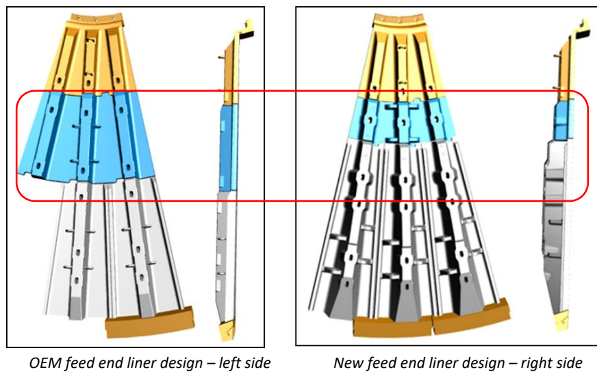
Figure 10 – Stage 1 Feed End Re-design Comparison
