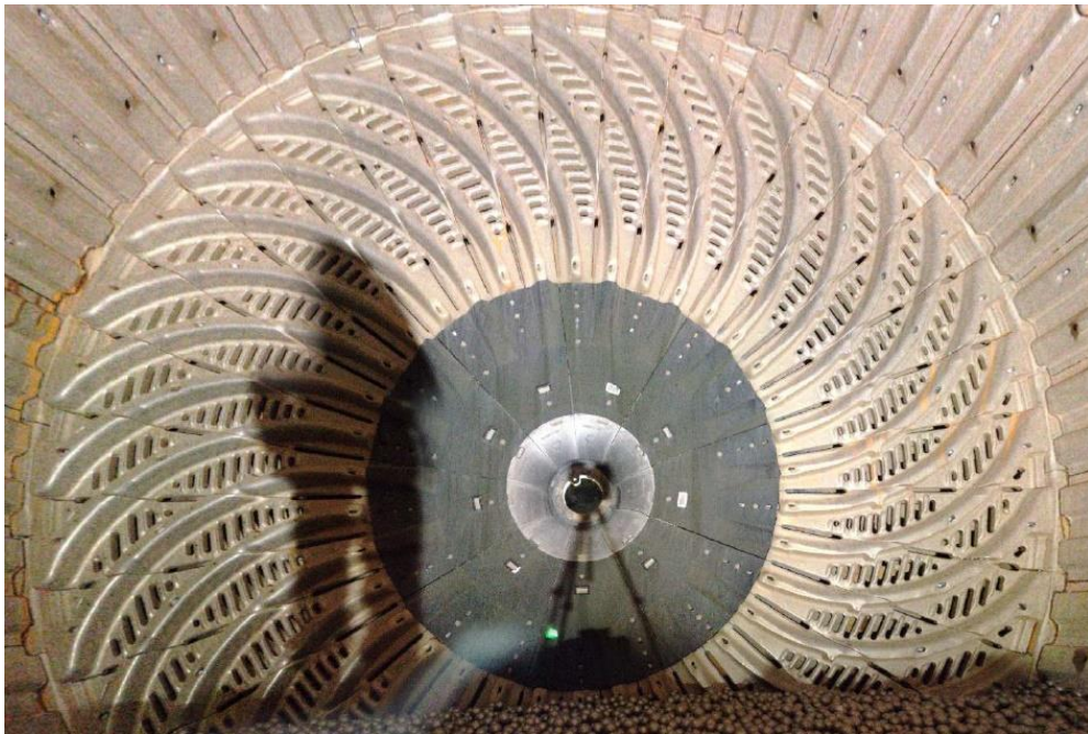
Figure 14 – The Super Vortex Discharge System
