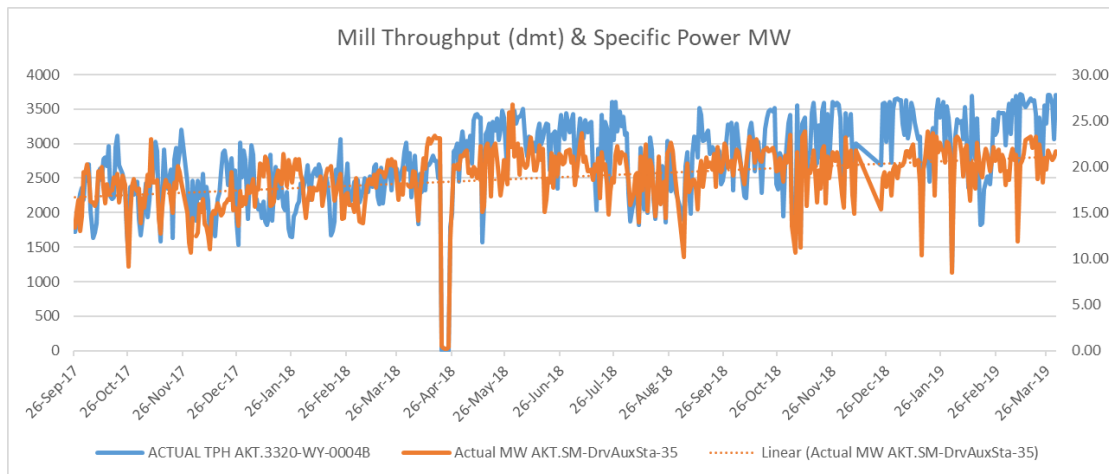
Figure 18 – SAG Mill Throughput and Specific Power
