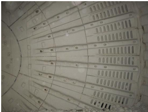
Figure 6 – Radial Discharge End Grate Design
