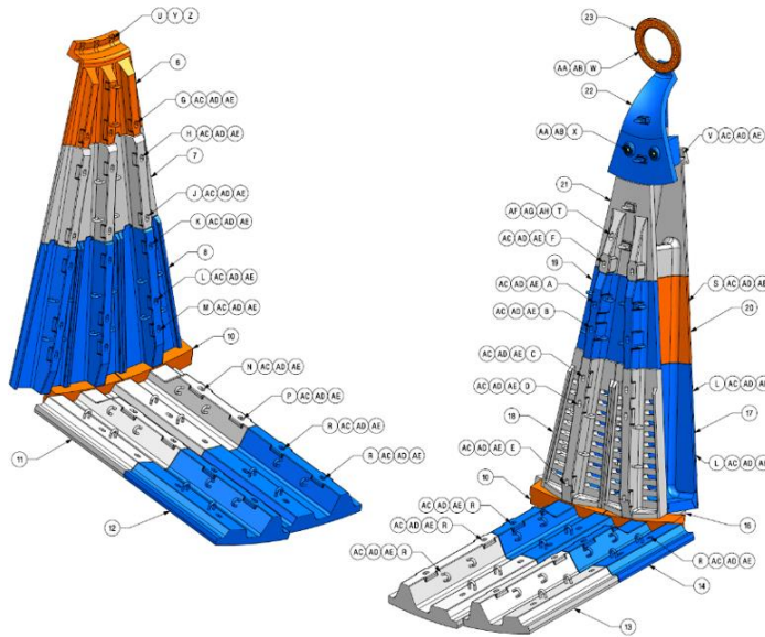
Figure 4 – OEM Liner Set General Assembly
