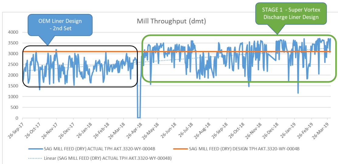
Figure 15 – SAG Mill Performance
