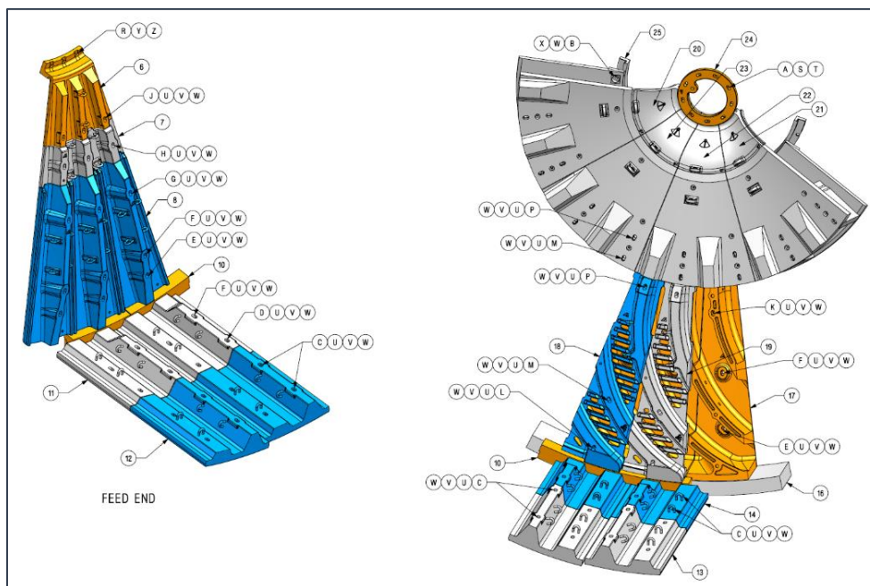
Figure 9 – Stage 1 Liner General Assembly
