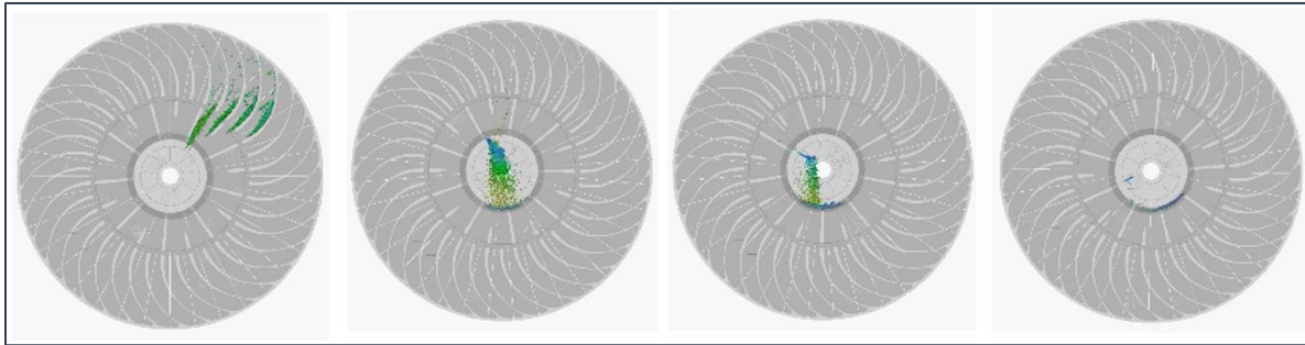
Figure 13 – DEM Results for the Super Vortex Discharge Design
