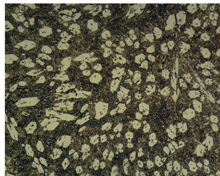
Duaplate D80 Microstructure
