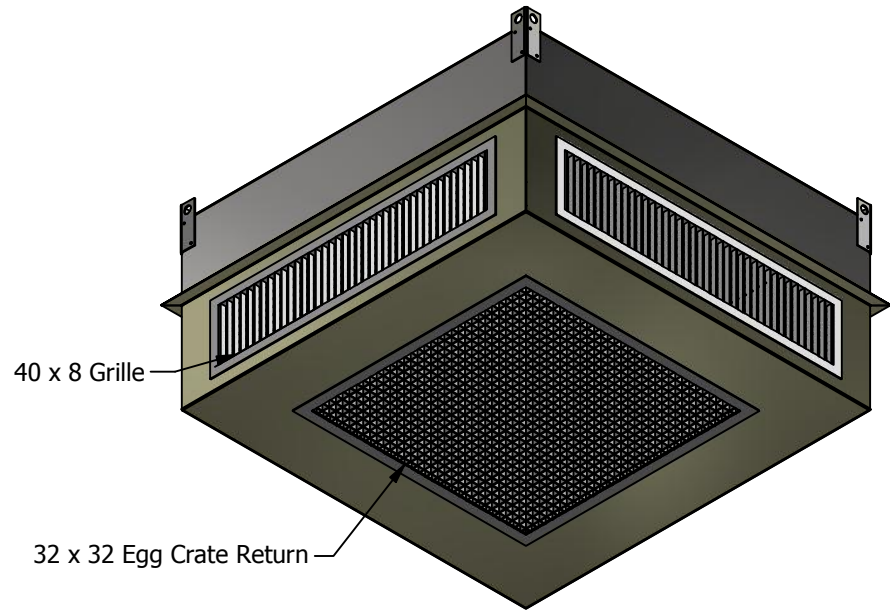
Concentric Diffuser System
