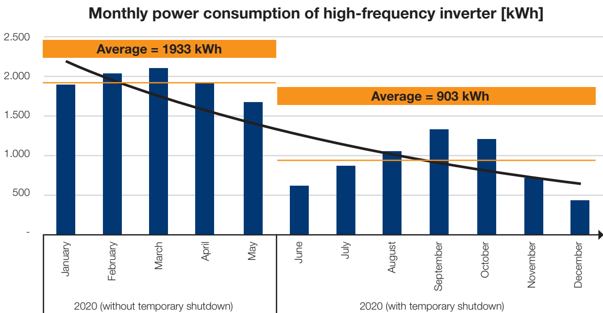
Figure 8: Monthly power consumption of the high-frequency converter in 2020
