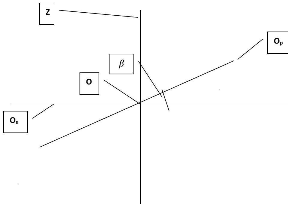
Figure 1: Cross section of the solar system.
