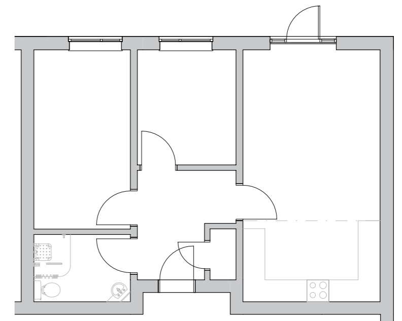
Apartment type B
