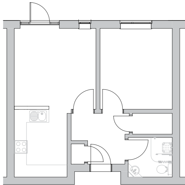
Apartment type A
