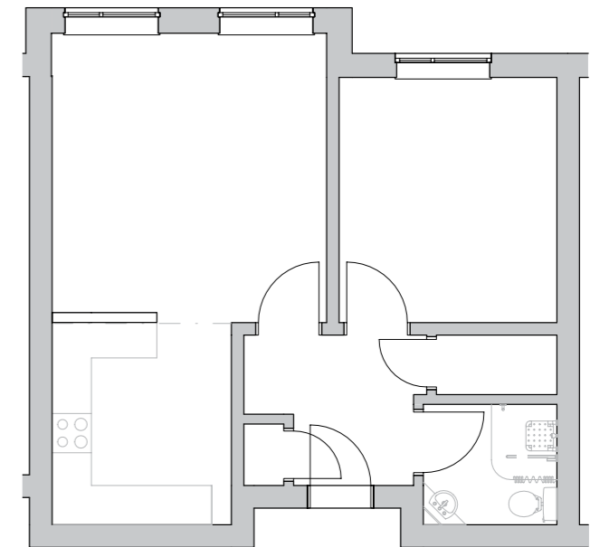
Apartment type A2
