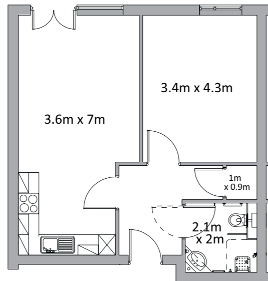
Apartment type B
