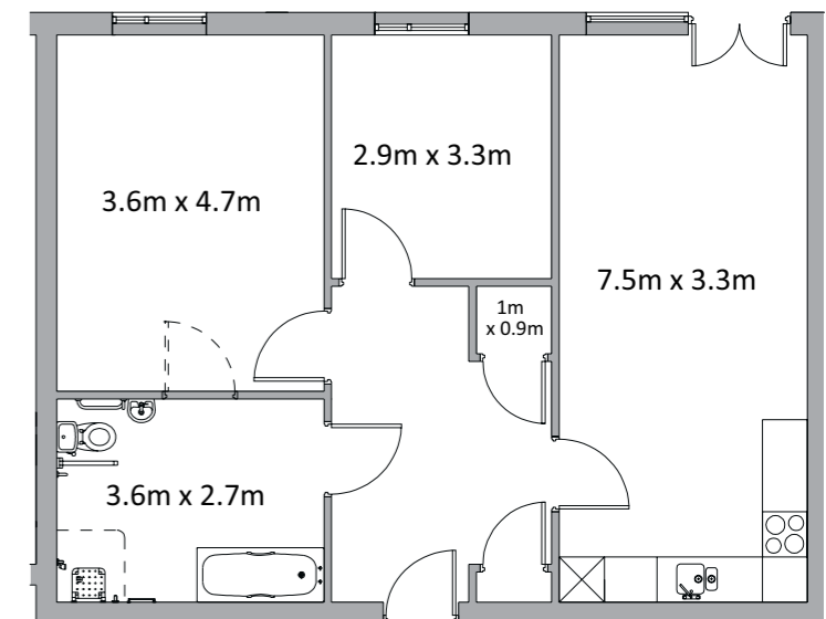
Apartment type H
