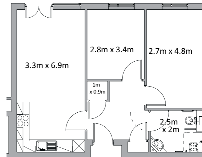
Apartment type G
