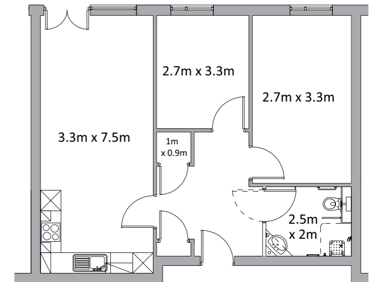
Apartment type D
