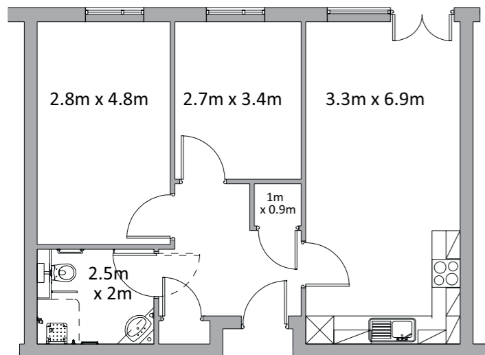
Apartment type E
