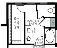
OPT. LINEN CLOSET AT MASTER BATH
