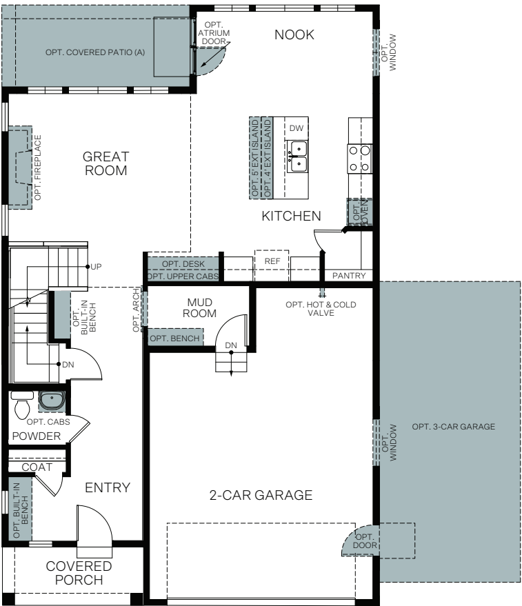
FIRST FLOOR 924 Sq. Ft.
