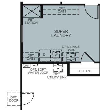
OPTIONAL SUPER LAUNDRY WITH PET STATION
