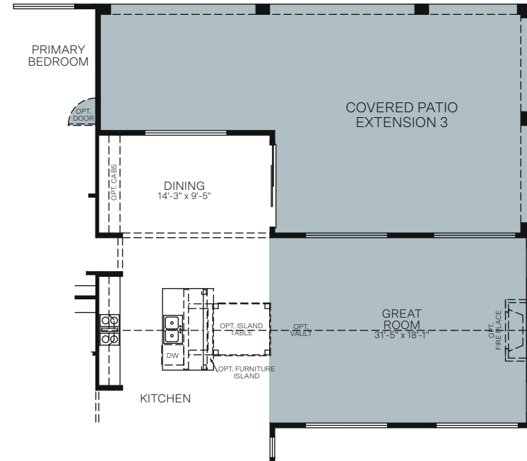
OPTIONAL COVERED PATIO EXTENSION 3 WITH GREAT ROOM EXTENSION (OPTIONAL DOOR AT PRIMARY BEDROOM ONLY AVAILABLE WITH COVERED PATIO EXTENSION 3)
