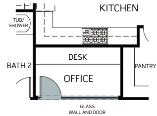
OPTIONAL GLASS WALL AND DOOR AT OFFICE
