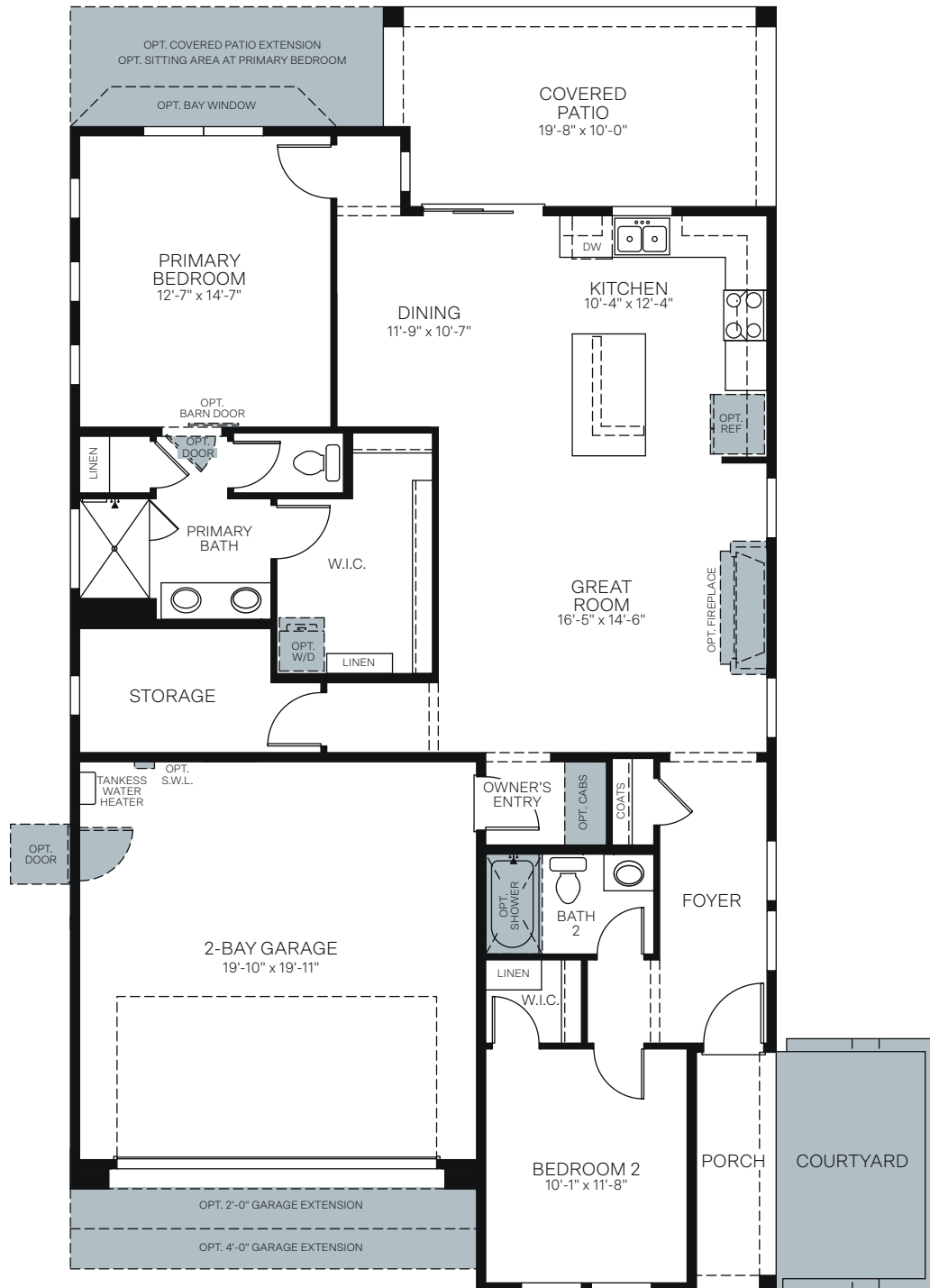
FLOOR PLAN
