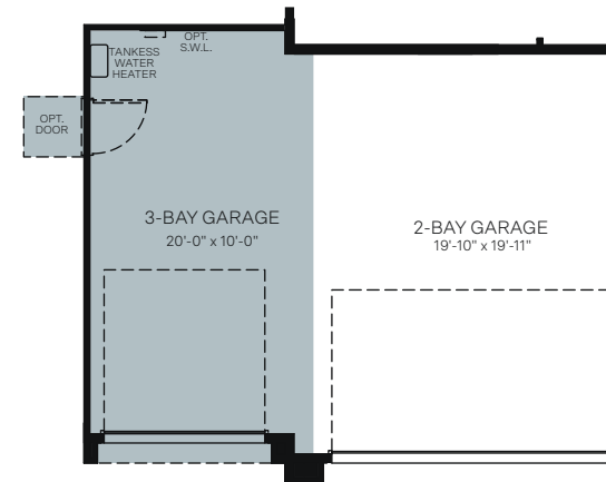
OPTIONAL 3-BAY GARAGE (LENGTH OF 3-BAY GARAGE DOES NOT EXTEND WITH 2'-0" AND 4'-0" GARAGE EXTENSIONS)
