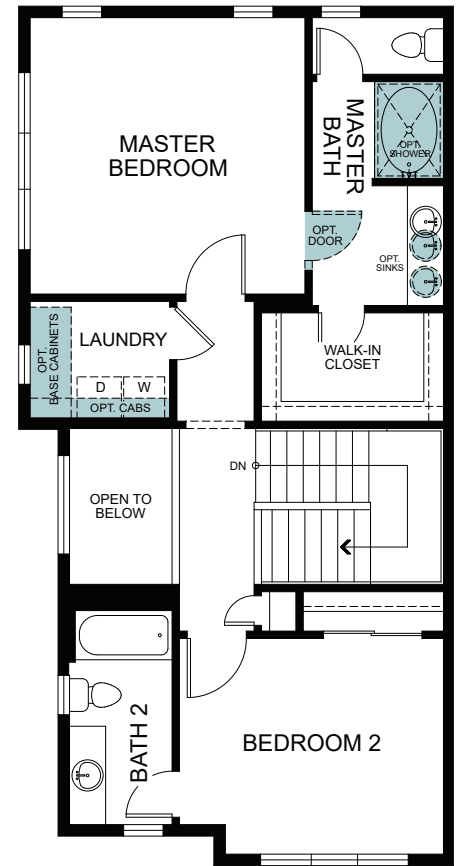
THIRD FLOOR 776 SQ. FT.
