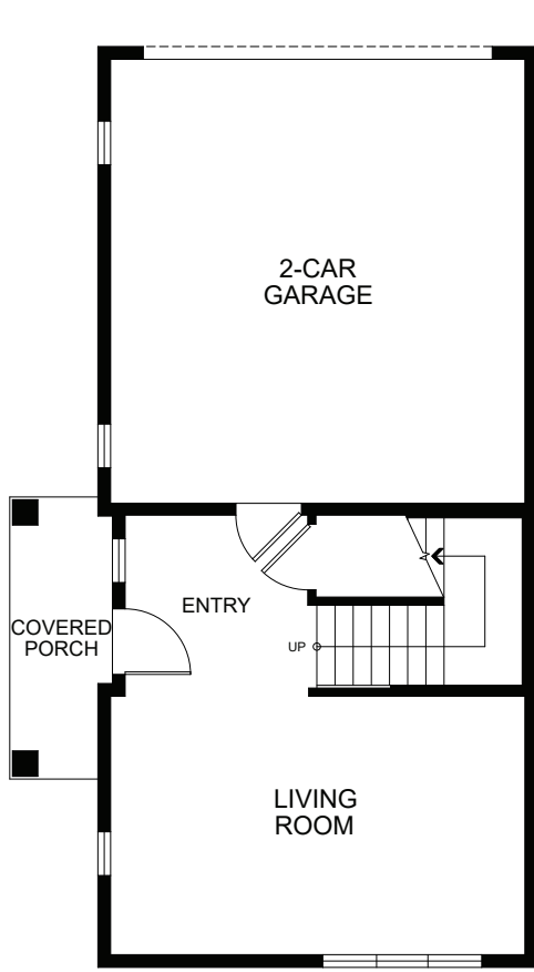
FIRST FLOOR 389 SQ. FT.
