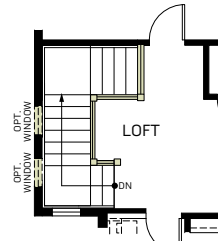
OPT. RAILING 4
