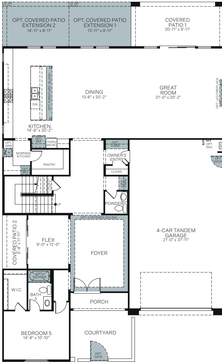
FIRST FLOOR
