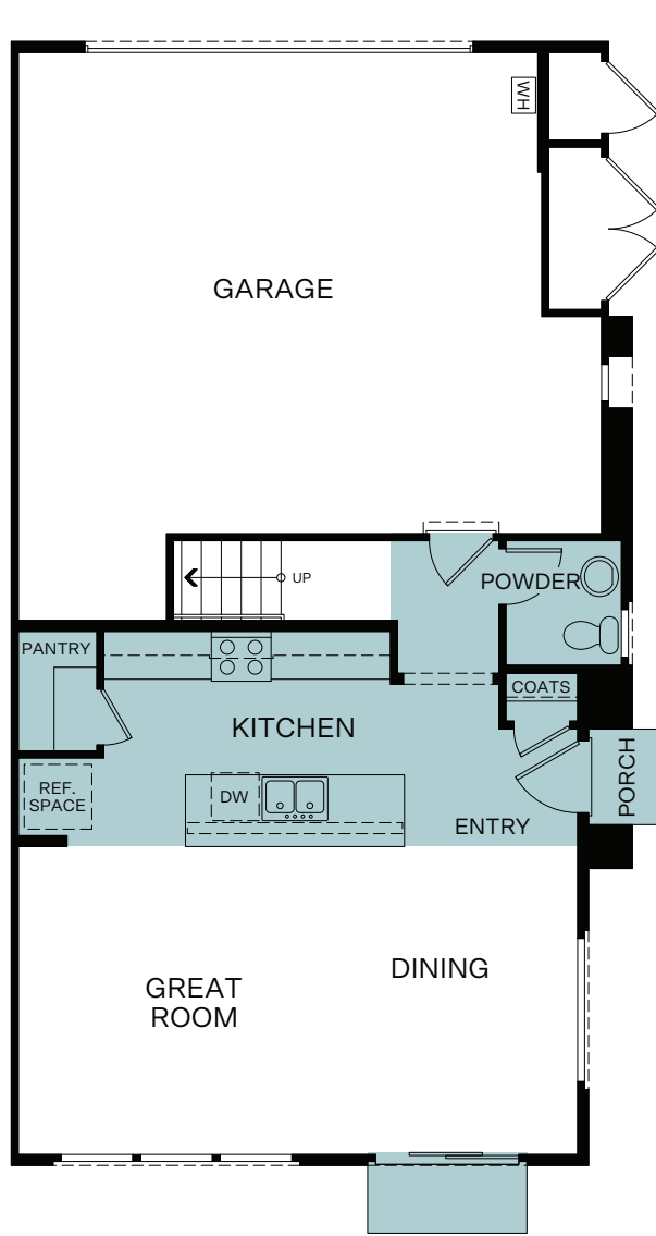
FIRST FLOOR
