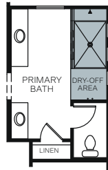
OPTIONAL EXTENDED SHOWER WITH HALF WALL AT PRIMARY BATHROOM
