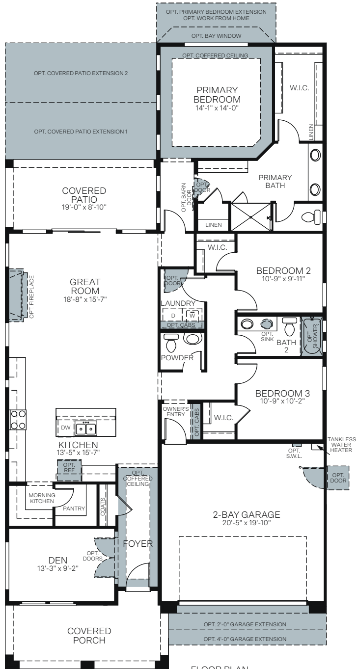
FLOOR PLAN
