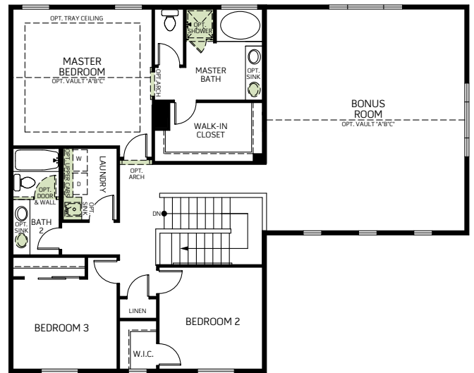
SECOND FLOOR 1,587 Sq. Ft.
