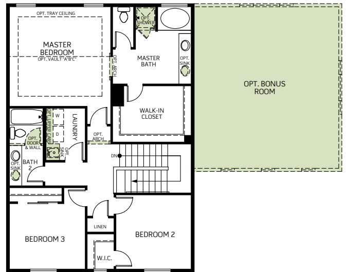
SECOND FLOOR 1,036 Sq. Ft.
