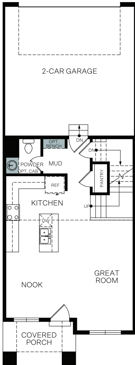
FIRST FLOOR 559 Sq. Ft.
