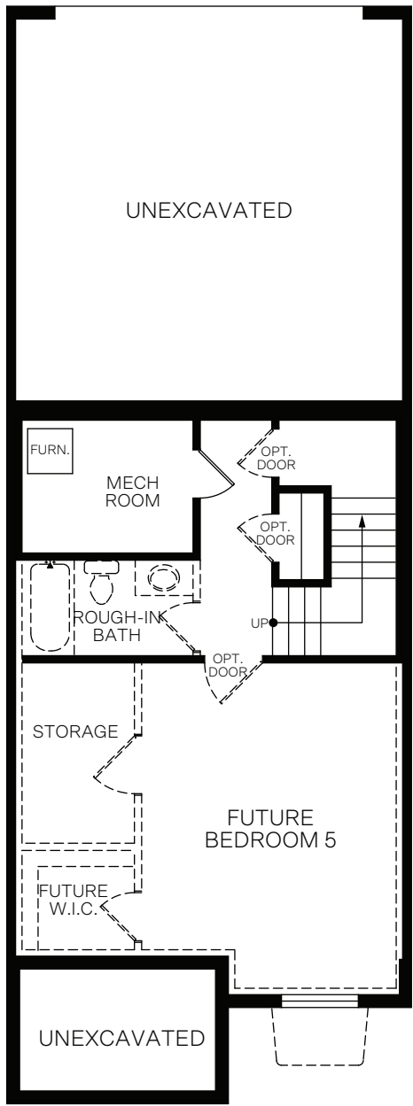
BASEMENT 586 Sq. Ft.
