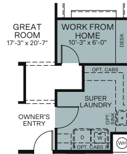
OPTIONAL SUPER LAUNDRY WITH WORK FROM HOME (NOT AVAILABLE WITH GUEST SUITE)
