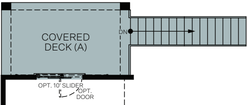
OPT. COVERED DECK (A) - FULL DAYLIGHT
