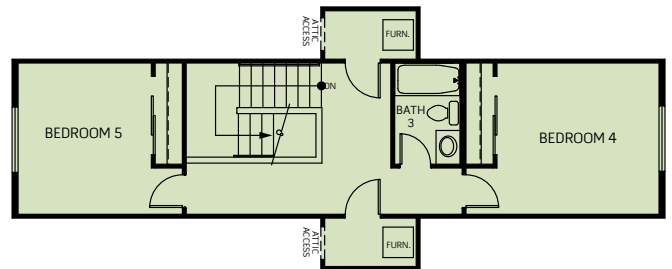
OPT. BONUS ROOM II WITH BEDROOM 4 & 5/ BATHROOM 3 Adds: 529 Sq. Ft.
