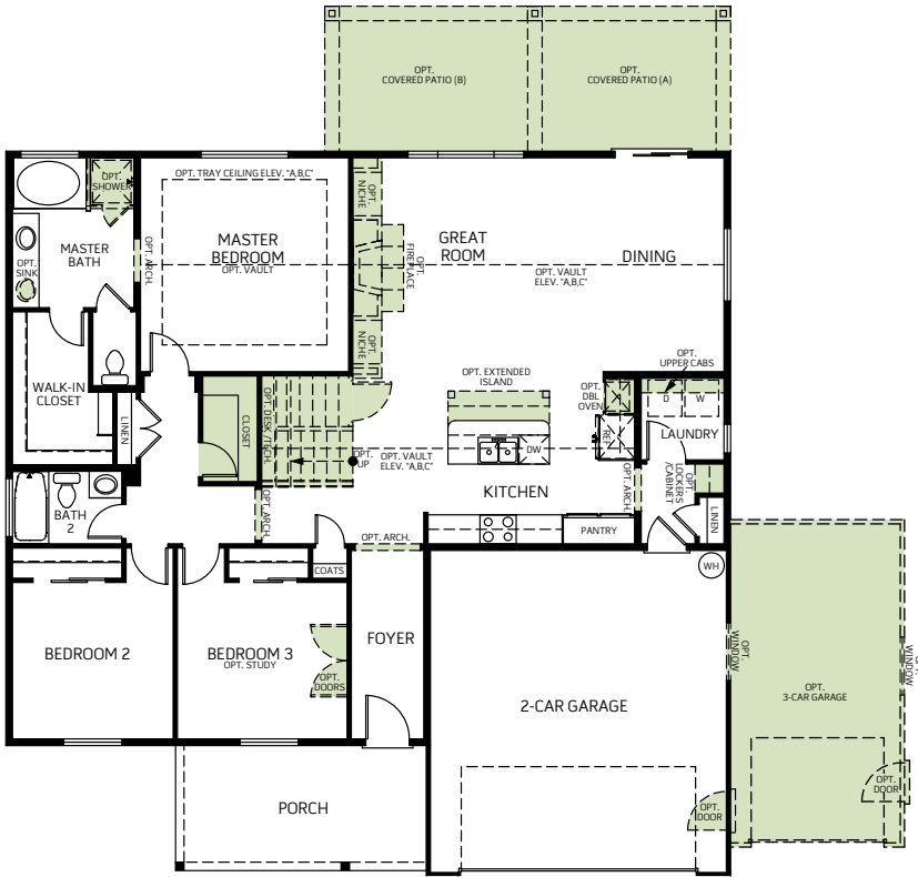
FIRST FLOOR 1,771 Sq. Ft.
